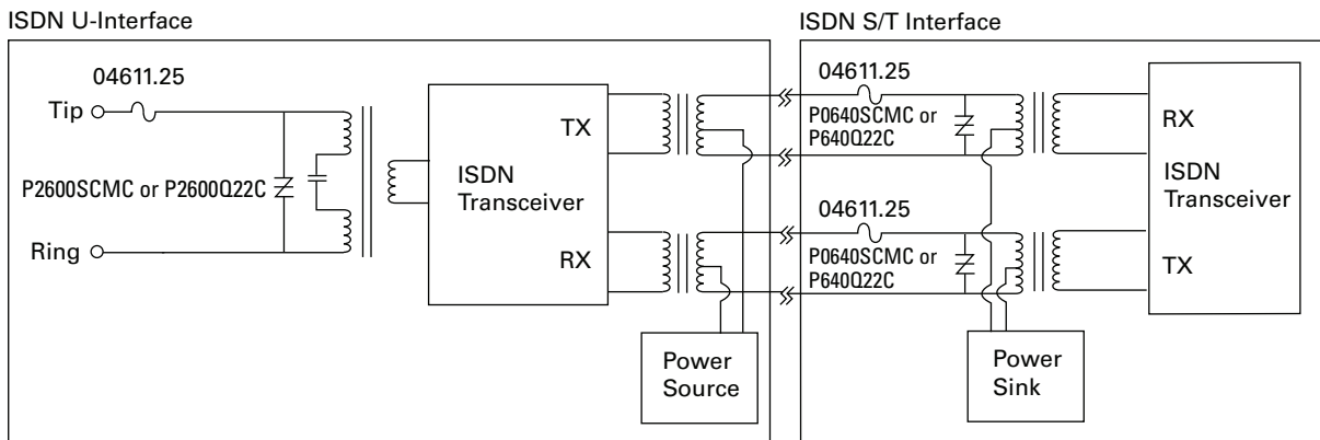
Figure 4.41 ISDN Protection
