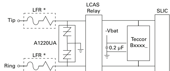
Figure 4.25 SLIC Protection with Limiting Resistance—Battrax
