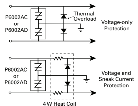
Figure 4.57 SIDACtor Cell Primary Protection
