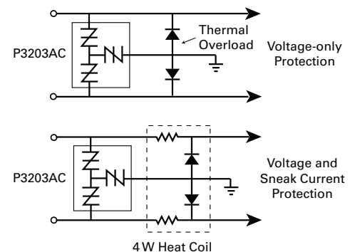
Figure 4.58 Balanced SIDACtor Primary Protection
